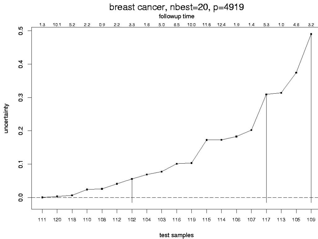
Fig. 4. Uncertainty plot for the predicted probabilities on the test set (19 samples) of the breast cancer prognosis data. The y-axis represents the uncertainty ( 1 - \text{predicted probability of } Y = 1 ), and the x-axis represents the 19 test samples sorted in increasing order of uncertainty. The follow-up time of patients is used to label the upper x-axis. The vertical bars represent classification errors, i.e. the test samples # 102, 117, 109 with follow-up times 3.3, 5.3, 3.2, respectively, were misclassified.
